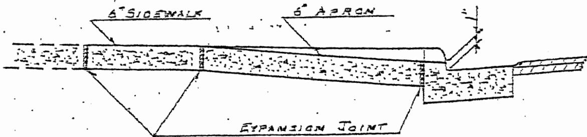
SECTION AA
